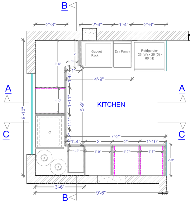
SECTIONAL PLAN BELOW PLATFORM
