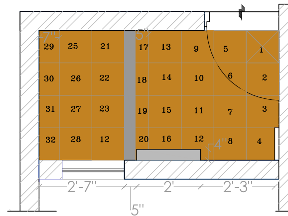
PLAN FOR TILING
