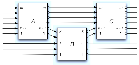
Figure 2: One stage in the construction of the adaptive sorting network. The original network B is “sandwiched” between the larger networks A and C .
