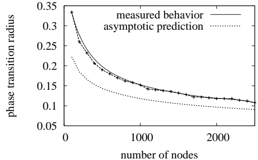
Fig. 9. Trilateration graph phase transition radius in G_n(r) .
