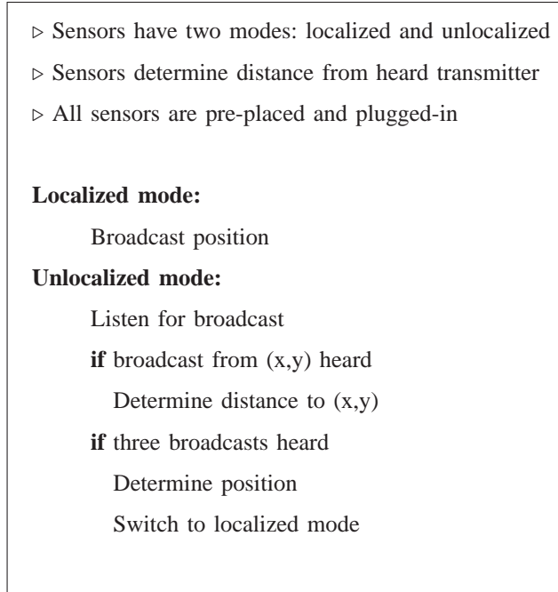
Fig. 7. The iterative trilateration protocol (ITP).
